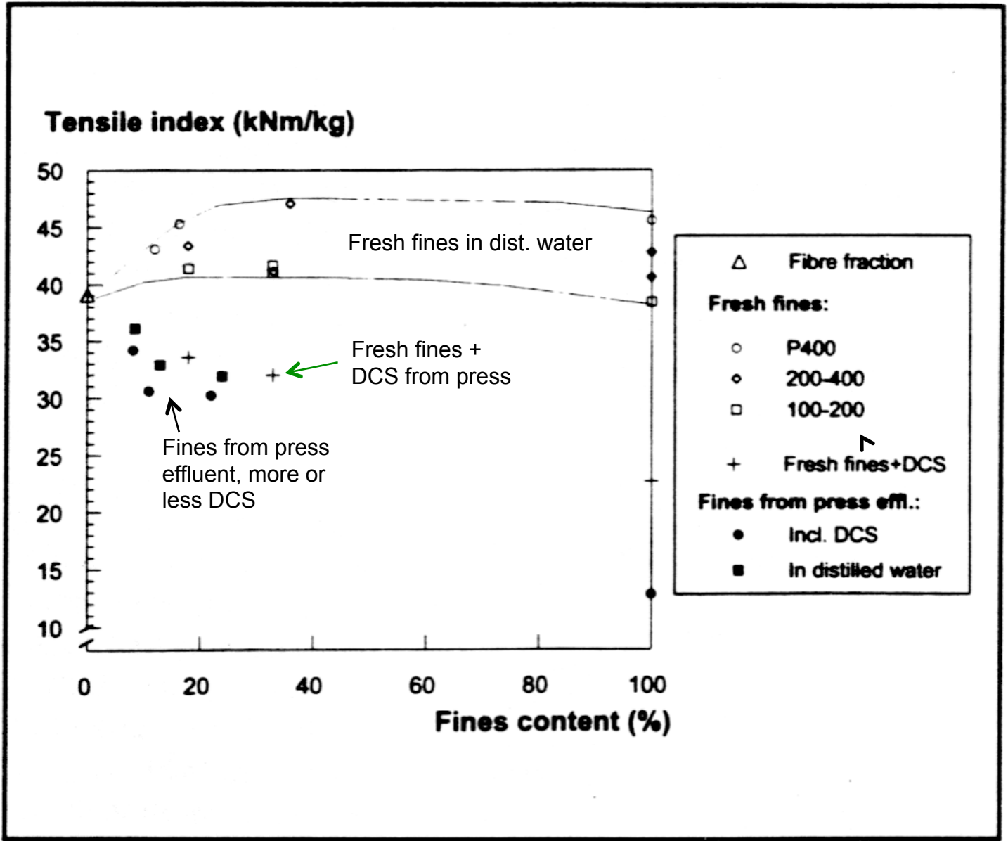
Fig. 9. Effect of the amount of DCS in the water phase during sheet making on the tensile index of handsheets containing bleached fines.
